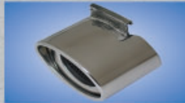
1x 150x95mm oval, 23° slash cut rolled with perforated insert
